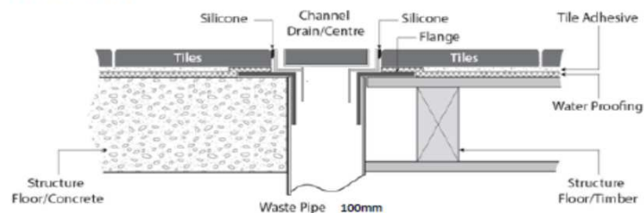
Installation Diagram
